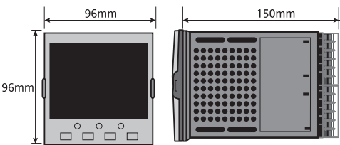
Panel cut-out 92mm (-0.0 +0.8) x 92mm (-0.0 +0.8)
